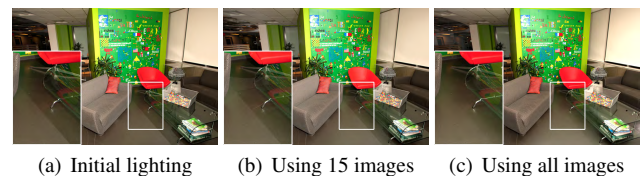
Figure 12: Our soft lighting modifier, applied to the lighting in (a) shows that a small number of images (15), even if carefully selected, do not provide enough close-by lights, needed for the gradual simulation of large area lights, (b). In (c) we show that the effect of our soft lighting modifier improves when used with the full image set.
