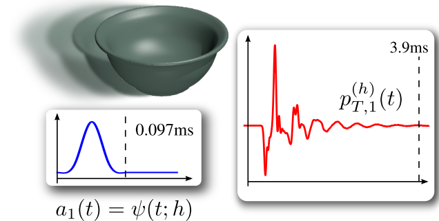
Figure 5: Precomputing directional pulses: We accelerate the bowl along its x -axis with an acceleration profile given by \psi(t; h) . This acceleration produces the pressure fluctuations p_{T,1}^{(h)}(t) at a listening position \mathbf{x} exterior to the object. We observe that pressure fluctuations at \mathbf{x} persist for much longer than the duration of \psi(t; h) due to acoustic reflections inside the bowl.
